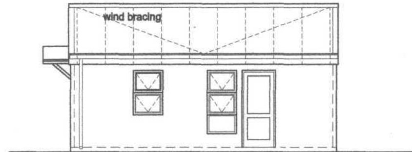
NORTH ELEVATION
